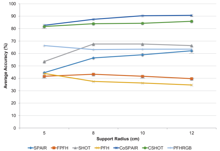
Figure 14: Leave-sequence-out instance-level average accuracy results for the Amazon Picking Challenge dataset.
